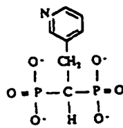
Risedronate
